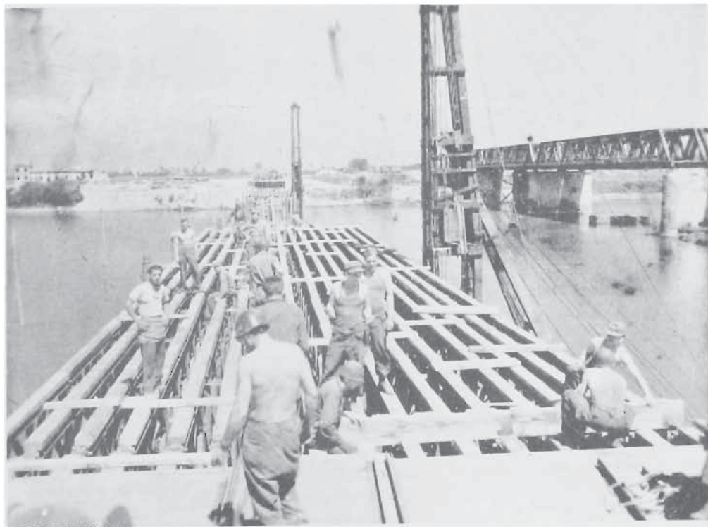
175TH BRIDGE ACROSS PO UNDER CONSTRUCTION
